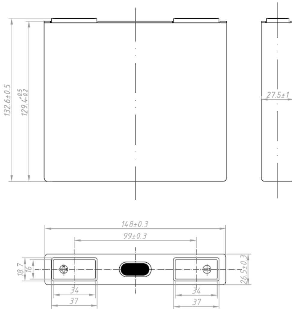
Drawing 1. Appearance and dimension of the battery
